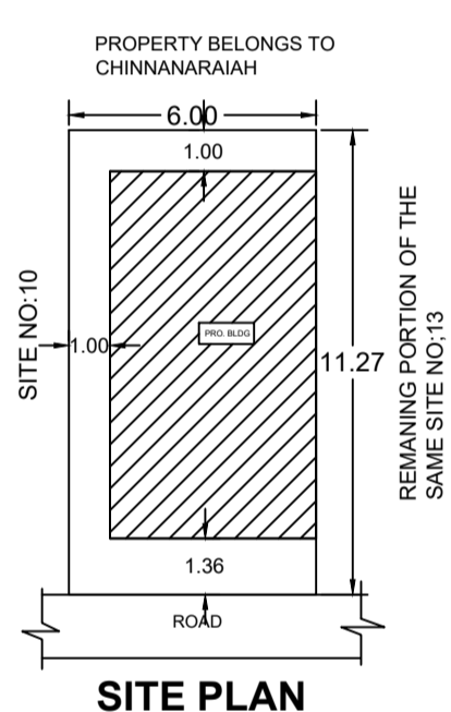
SITE PLAN
