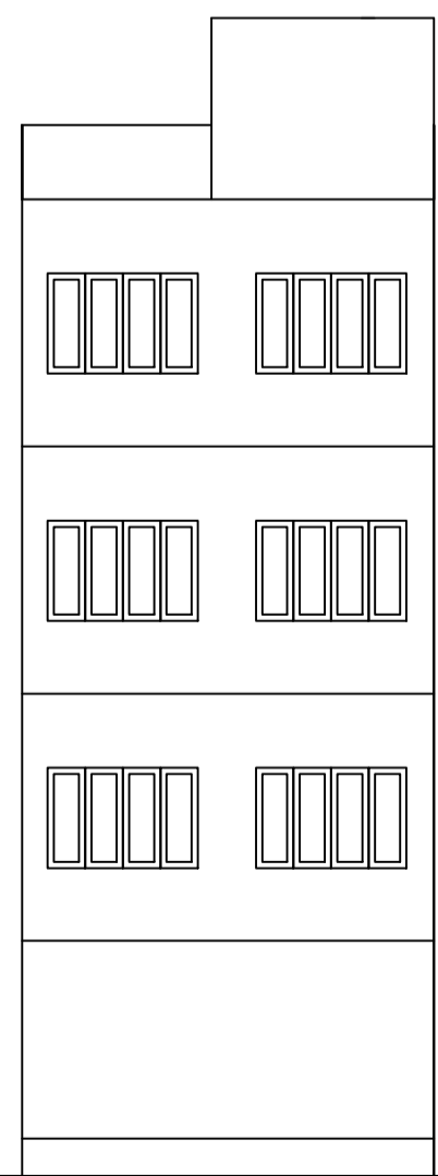
FRONT ELEVATION
